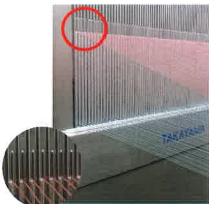
Enlarged Picture of Leasing Area
