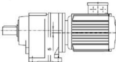
H.1500.12.5 Motor f trash transport incl. gearbox
